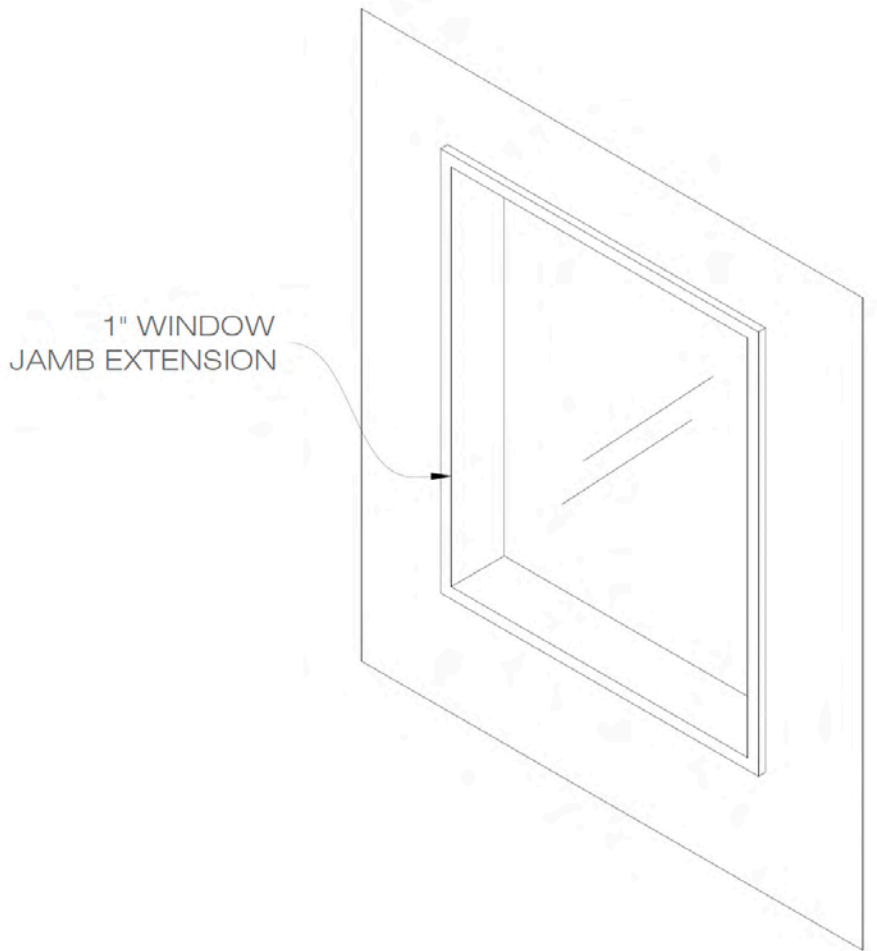
WINDOW DETAIL
